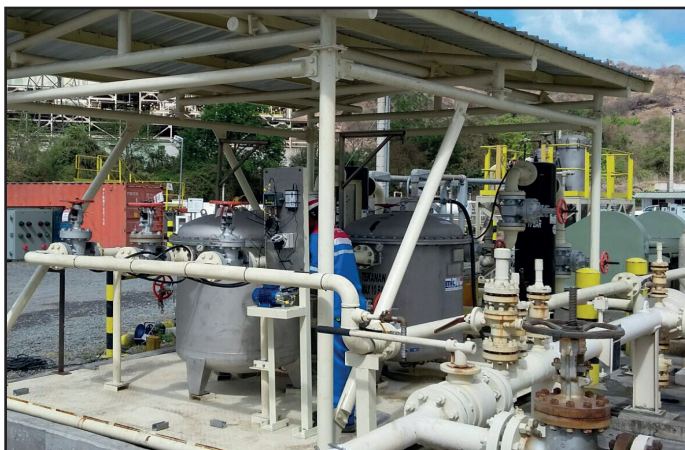
Changing 1 \mu m high flow filter elements HF900 after 16.000.000 l.
