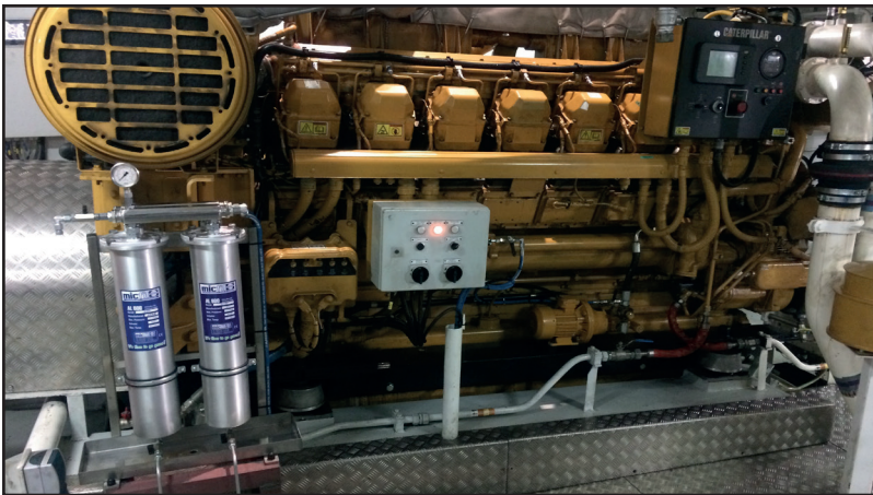
AL600 double system for oil on a generator
